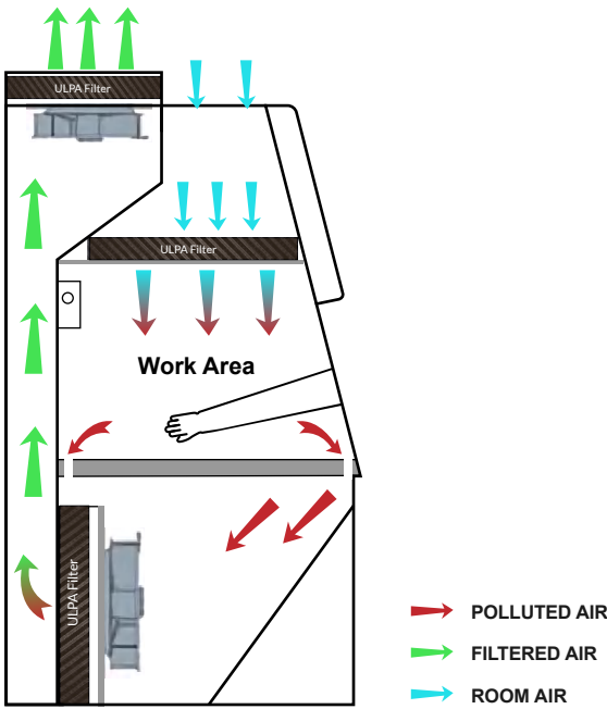
Airflow Pattern
